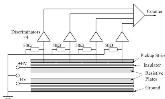
Fig. 1. The design of prototype RPCs for the BESIII spectrometer.
