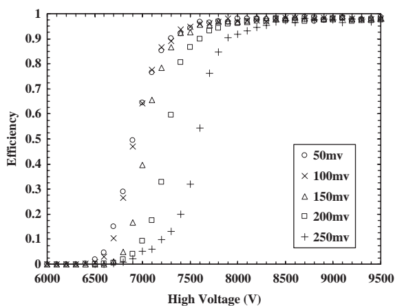
Fig. 7. Efficiencies versus high voltage for different discrimination thresholds.
