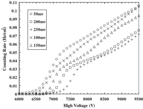
Fig. 8. Singles counting rates versus high voltage for different discrimination thresholds.
