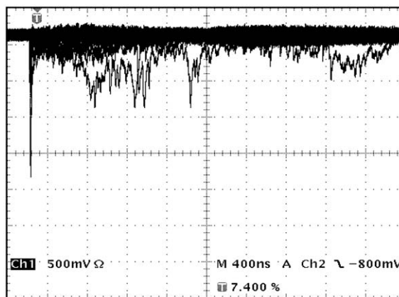
Fig. 11. Oscilloscope traces of 20 triggered cosmic ray muon signals recorded in RPC at 12 kV. The horizontal scale is 400 ns/div. and the vertical scale is 500 mV/div. Some pulses can be as large as a few volts and can last several microseconds with multiple secondary streamers.
