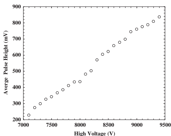
Fig. 6. Average signal amplitudes versus the high voltage.
